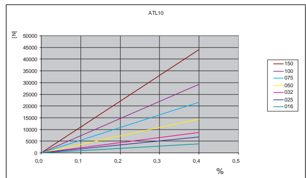
Load / Elongation [ % ]
